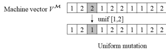
Fig. 6. Mutation operators.
